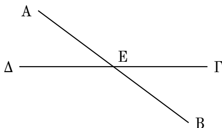
Figure 1.3.: Vertical angles are equal
