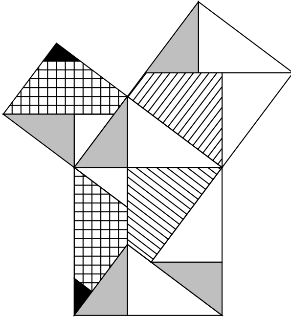
Figure 3.1.: The Pythagorean Theorem
