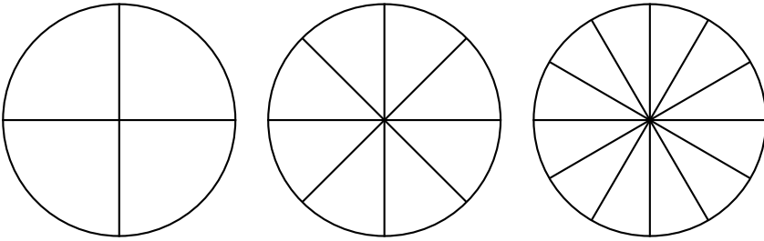
Figure 1.1.: The diameter divides the circle
