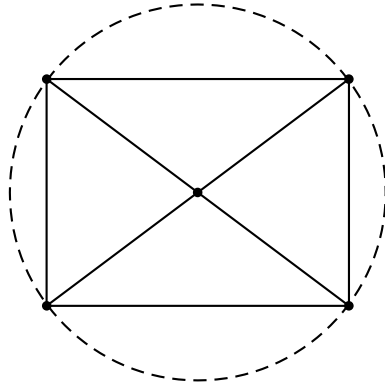
Figure 1.5.: Right angles inscribed in a circle
