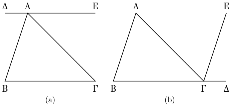
Figure 1.4.: Euclid's I.32, by the Pythagoreans and himself
