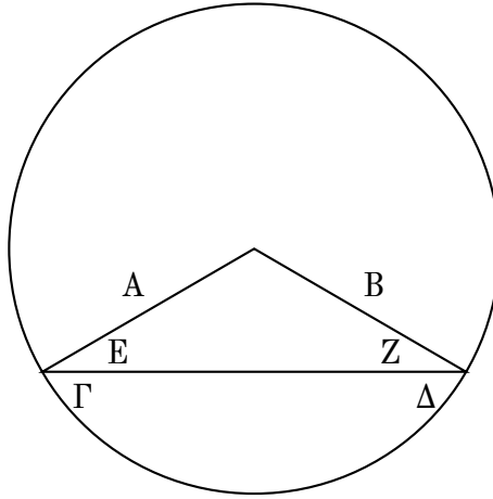
Figure 1.2.: Aristotle's proof of Euclid I.5
