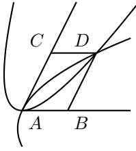
Figure A.5. Two intersecting parabolas
