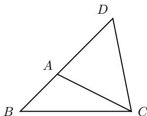
Figure 1.5. Euclid's I.20
