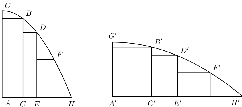
Figure 6.4. Proportional areas
