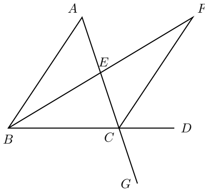
Figure 1.2. Euclid's I.16
