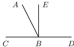
Figure 1.1. Euclid's I.12
