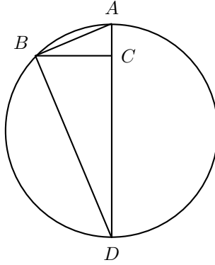
Figure 6.5. Uniform circular motion
