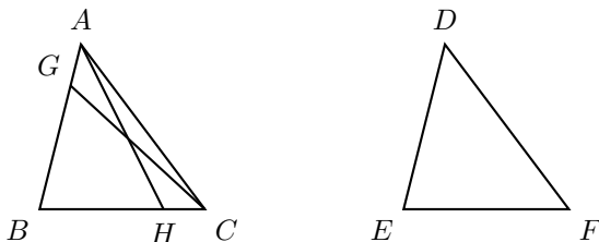
Figure 1.8. Euclid's I.26
