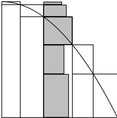
Figure 6.3. Newton's quadrature
