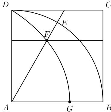
Figure 5.4. The quadratrix
