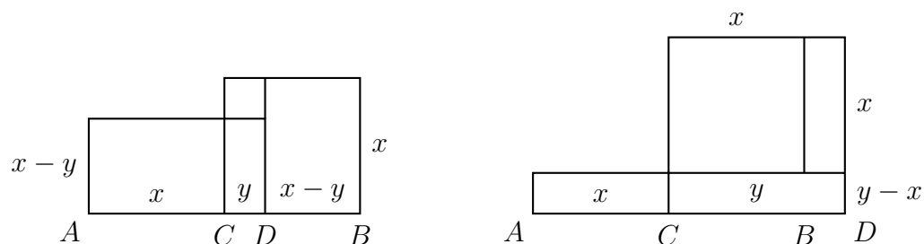
Figure 3.1. Quadratic equations as in Euclid
