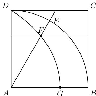
Figure 5.3. The quadratrix
