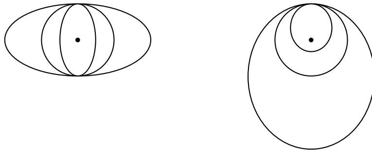
Figure 6.6. Various orbits
