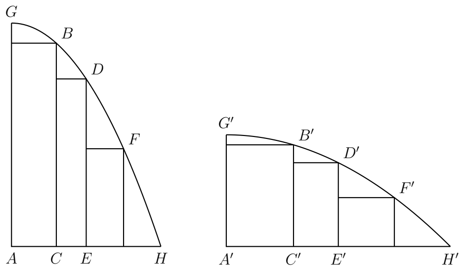
Figure 6.4. Proportional areas
