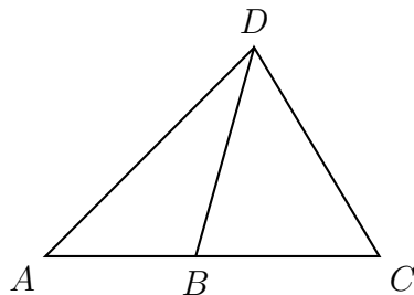
Figure 5.1. Ratios in triangles
