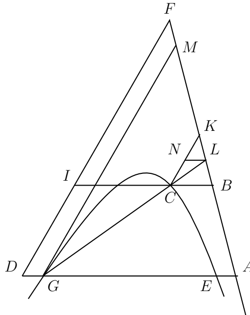
Figure 6.1. Descartes's construction of a hyperbola
