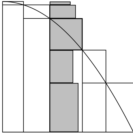
Figure 6.3. Newton's quadrature
