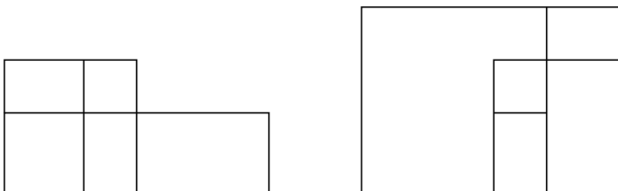
Figure 3.2. A quadratic equation as in al-Khwārizmī
