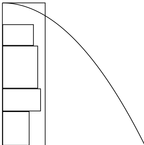
Figure 6.2. Unclear quadrature
